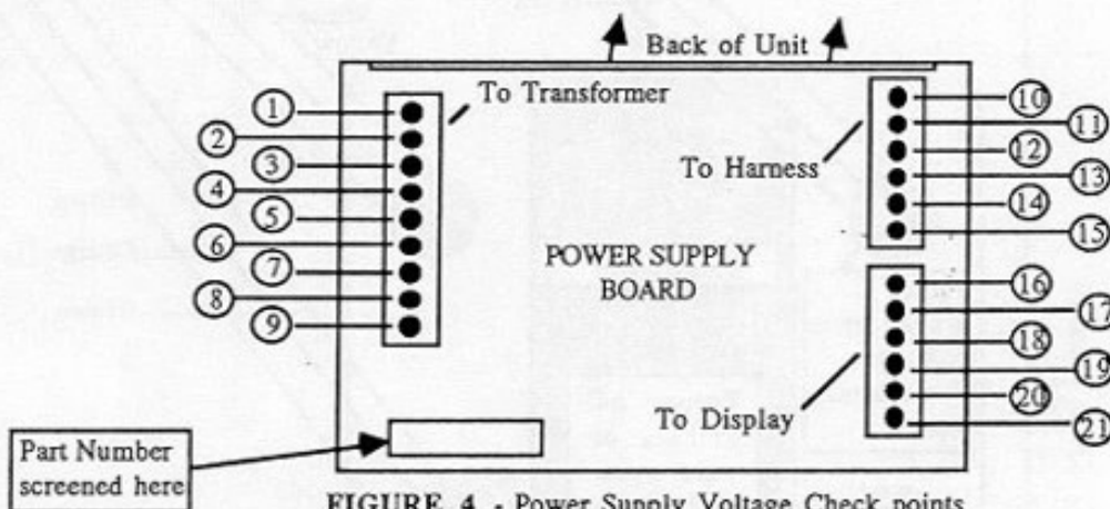
FIGURE 4 - Power Supply Voltage Check points (ESQ-1 Metal)
