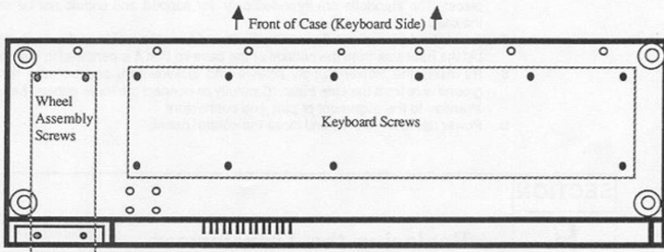
FIGURE 10--Bottom of ESQ-1 Plastic Case
