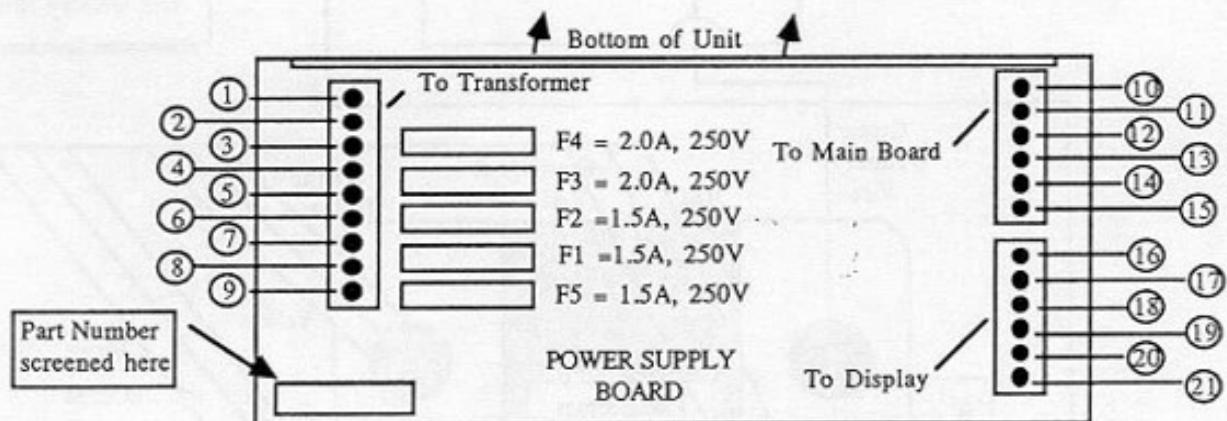
FIGURE 13 Power Supply Voltage Check points (ESQ-M)
